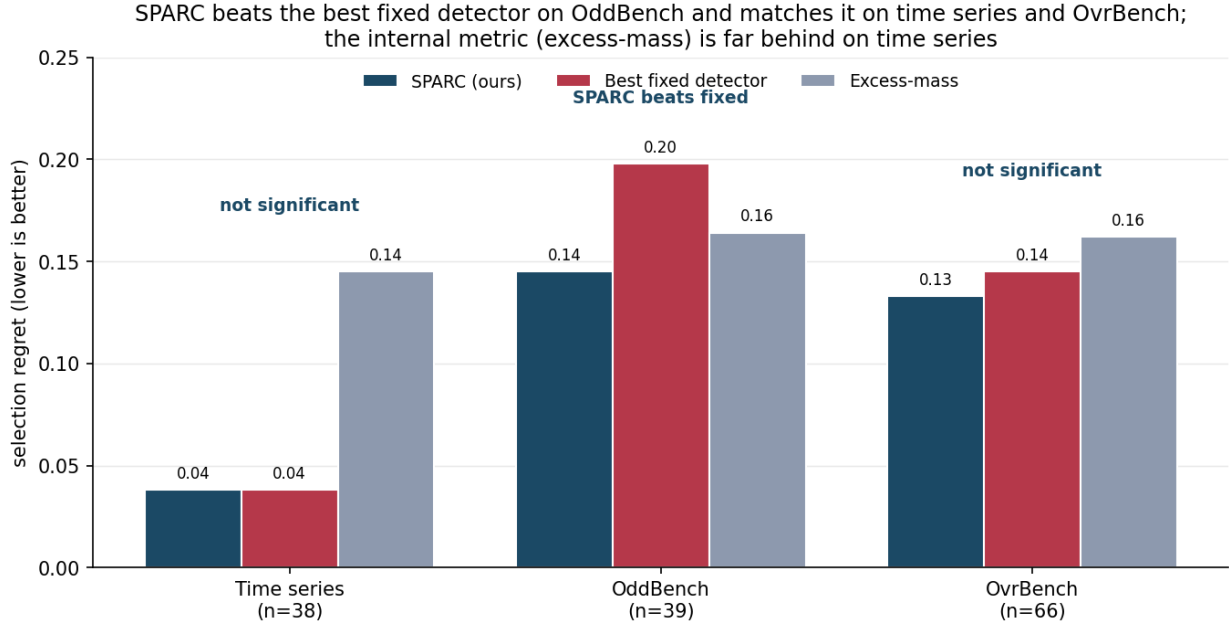
Figure 7. Selection regret by data source for SPARC versus the best fixed detector and excess-mass. SPARC significantly beats the fixed detector on OddBench ( p = 0.021 ) and does not significantly differ from it on time series ( p = 0.56 ) or OvrBench ( p = 0.42 ); the internal criterion is far behind on time series. Significance is the paired Wilcoxon test of SPARC against the fixed detector.
