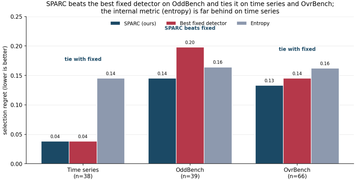
Figure 7. Selection regret by modality for SPARC versus the best fixed detector and entropy. SPARC significantly beats the fixed detector on OddBench ( p = 0.021 ) and ties it on time series and OvrBench; the internal criterion is far behind on time series. Significance is the paired Wilcoxon test of SPARC against the fixed detector.
