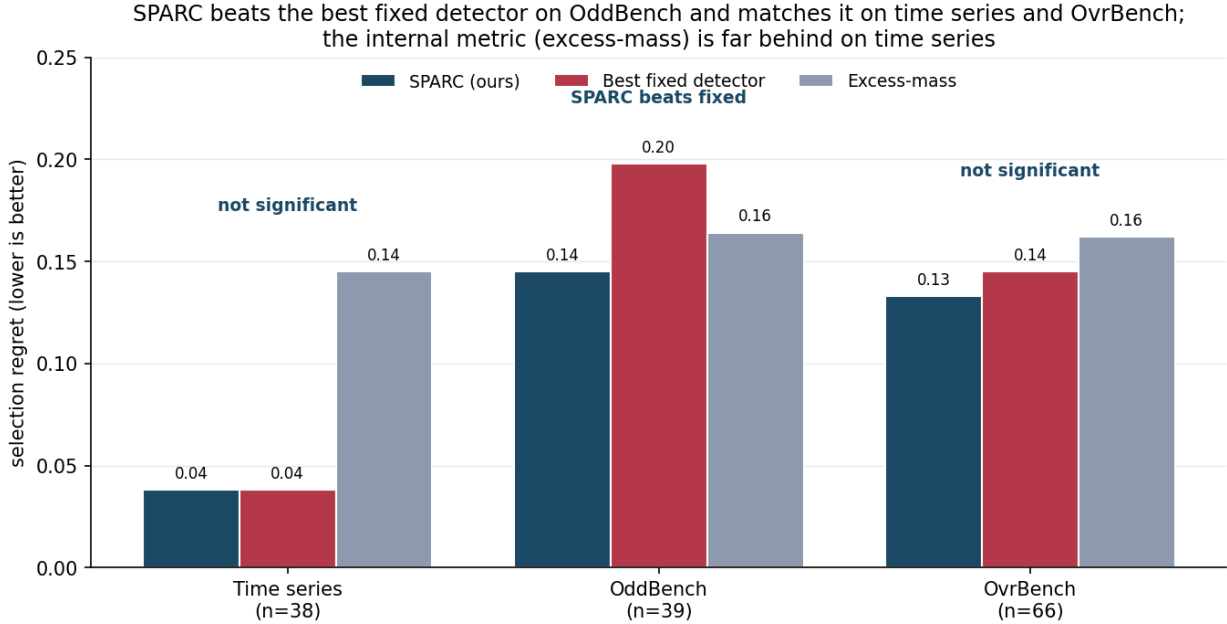
Figure 7. Selection regret by data source for SPARC versus the best fixed detector and excess-mass. SPARC significantly beats the fixed detector on OddBench ( p = 0.021 ) and does not significantly differ from it on time series ( p = 0.56 ) or OvrBench ( p = 0.42 ); the internal criterion is far behind on time series. Significance is the paired Wilcoxon test of SPARC against the fixed detector.
