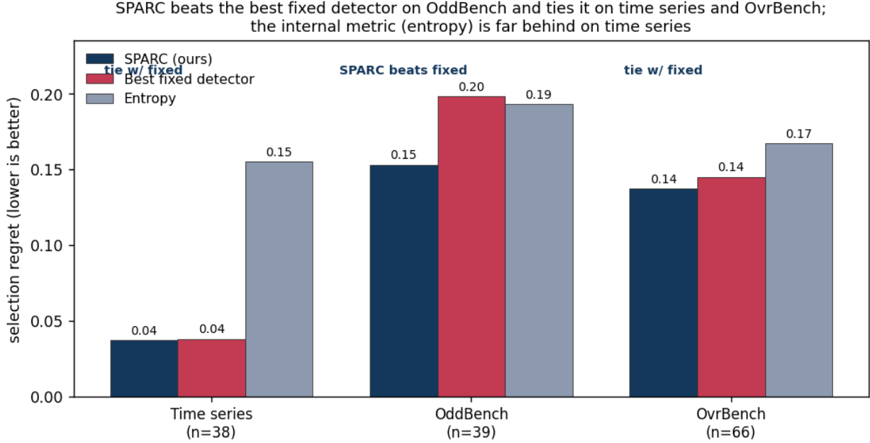
Figure 7. Selection regret by modality for SPARC versus the best fixed detector and entropy. SPARC significantly beats the fixed detector on OddBench ( p = 0.029 ) and ties it on time series and OvrBench; the internal criterion is far behind on time series. Significance is the paired Wilcoxon test of SPARC against the fixed detector.
