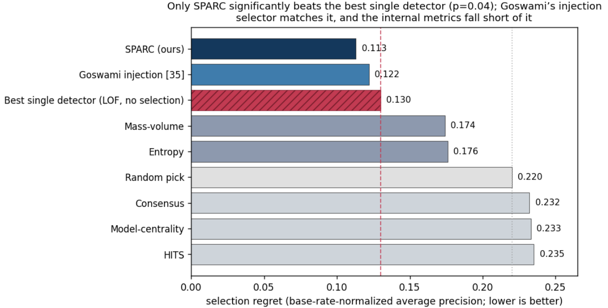
Figure 6. Model-selection regret on the 151-task ADReal benchmark (base-rate-normalized average precision; lower is better). The dashed line is the best fixed detector (LOF, k = 10 , no per-task selection), the bar every selection method must beat; the dotted line is a random pick. SPARC is the only method that significantly beats the fixed detector; Goswami’s injection selector matches it; entropy and mass-volume fall short of it; the agreement selectors fall below random.
