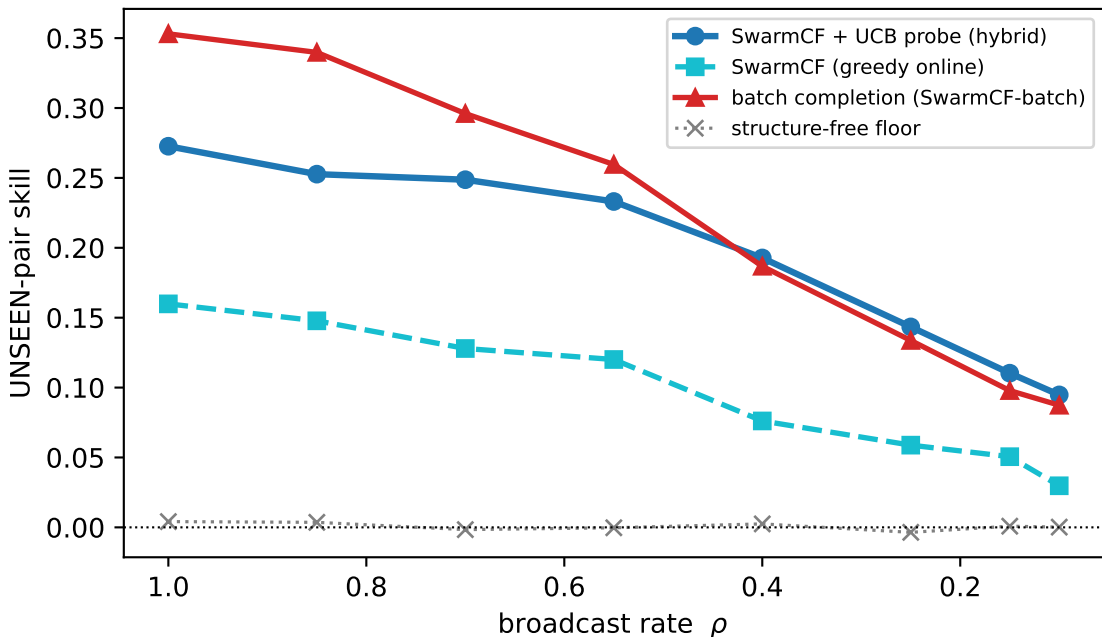
All-tasks menu ( c = n ): a UCB probe restores the online estimator's lead over batch completion that pure greedy selection gives up
