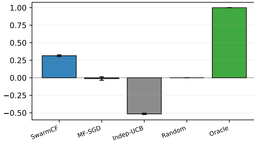
(b) Earned (anytime) skill
