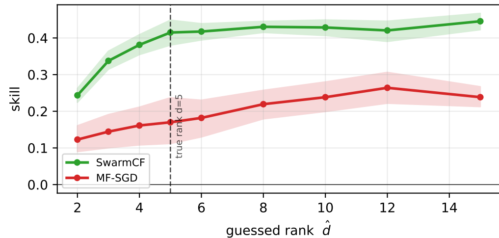
Earned (anytime) skill
