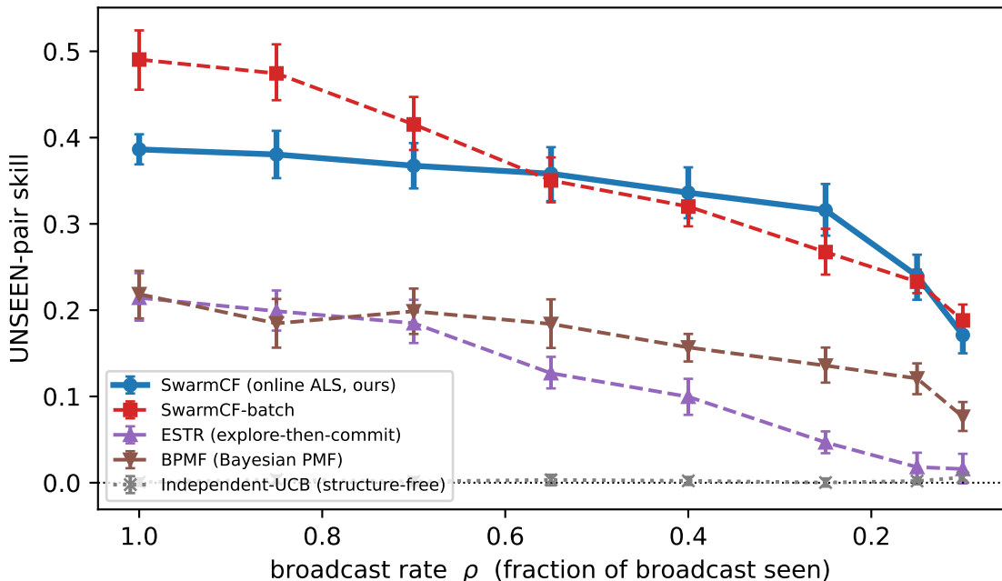
Masking-robustness (unseen-pair skill): our online SwarmCF stays robust as the broadcast is masked; batch methods (SwarmCF-batch/ESTR/BPMF) decay
