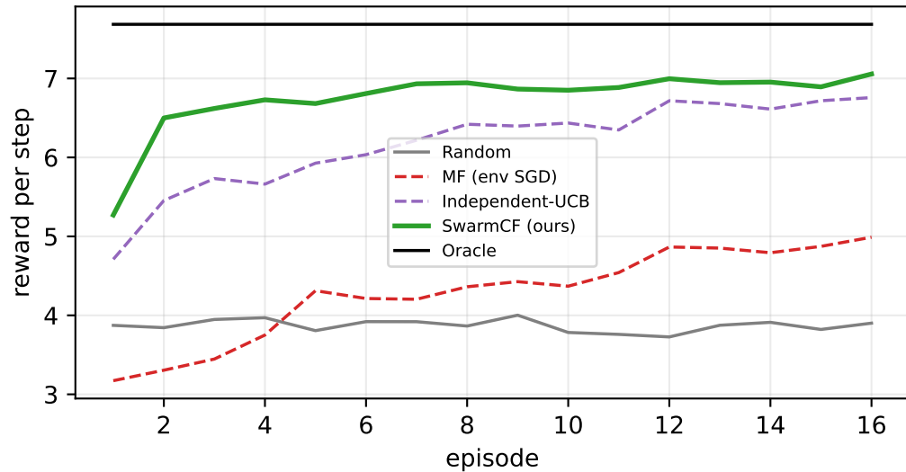
Learning curves
