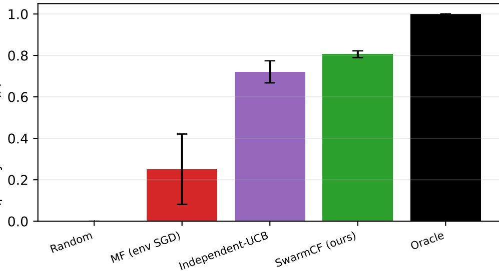
Converged skill
