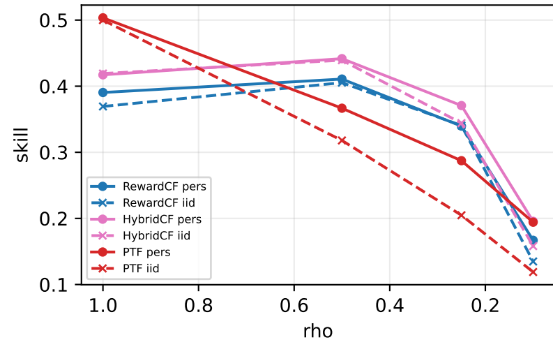
unseen skill: persistent vs iid
