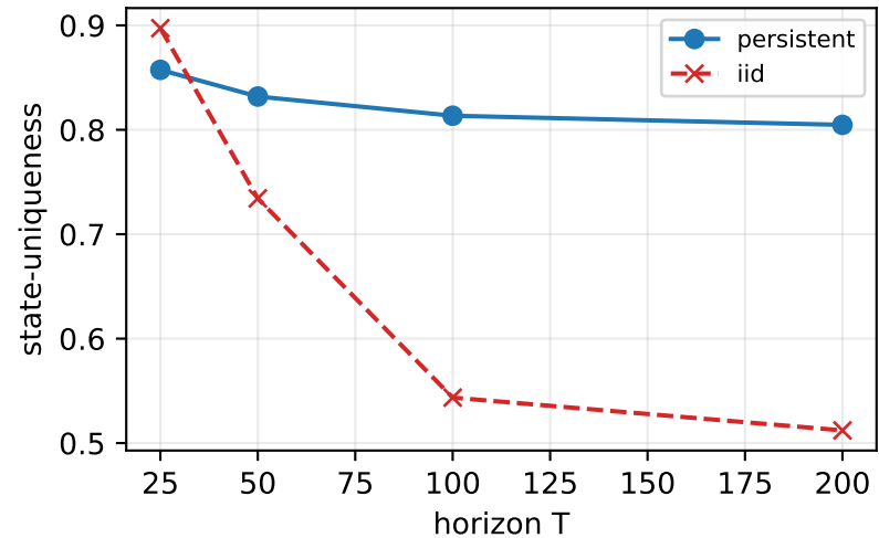
decentralization durability (rho=0.25) persistent durable, iid transient
