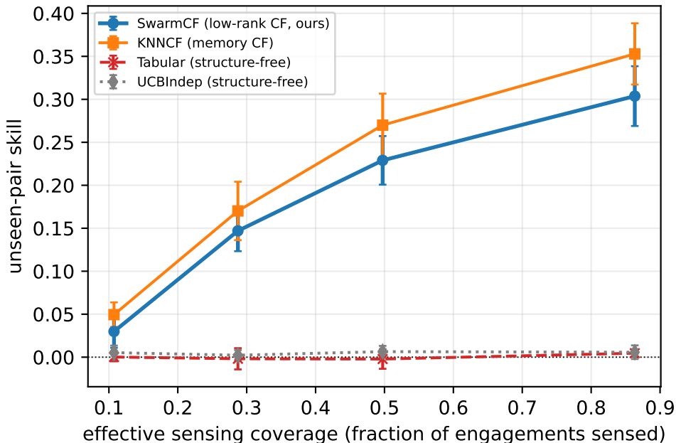
Sensing-grounded observability: the categorical win survives geometry-limited, distance-noisy sensing (masking emergent from physics)
