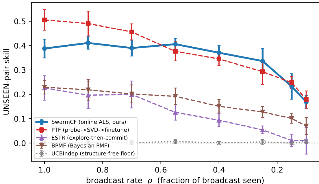
Masking-robustness (unseen-pair skill): our online SwarmCF stays robust as the broadcast is masked; batch-SVD hybrids (PTF/ESTR/BPMF) decay
