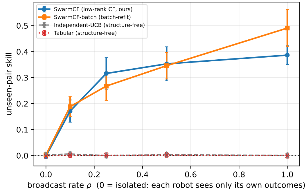
(a) Collaboration value: the comms-free broadcast unlocks generalization for low-rank CF, is worthless to structure-free
