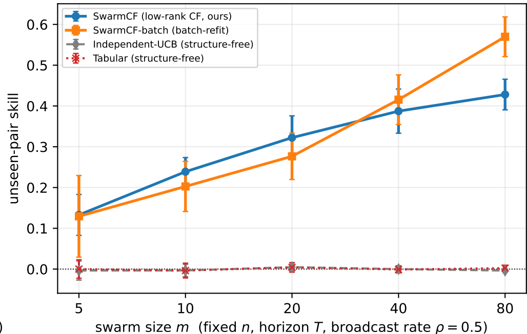
(b) Positive scaling: the swarm gets SMARTER as it grows; more robots feed the SHARED structure; structure-free stays flat
