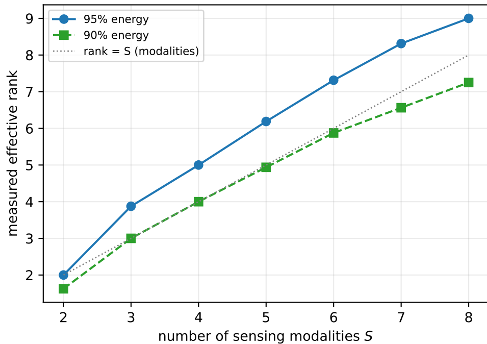
(b) Effective rank tracks the modality count ( n=240 )
