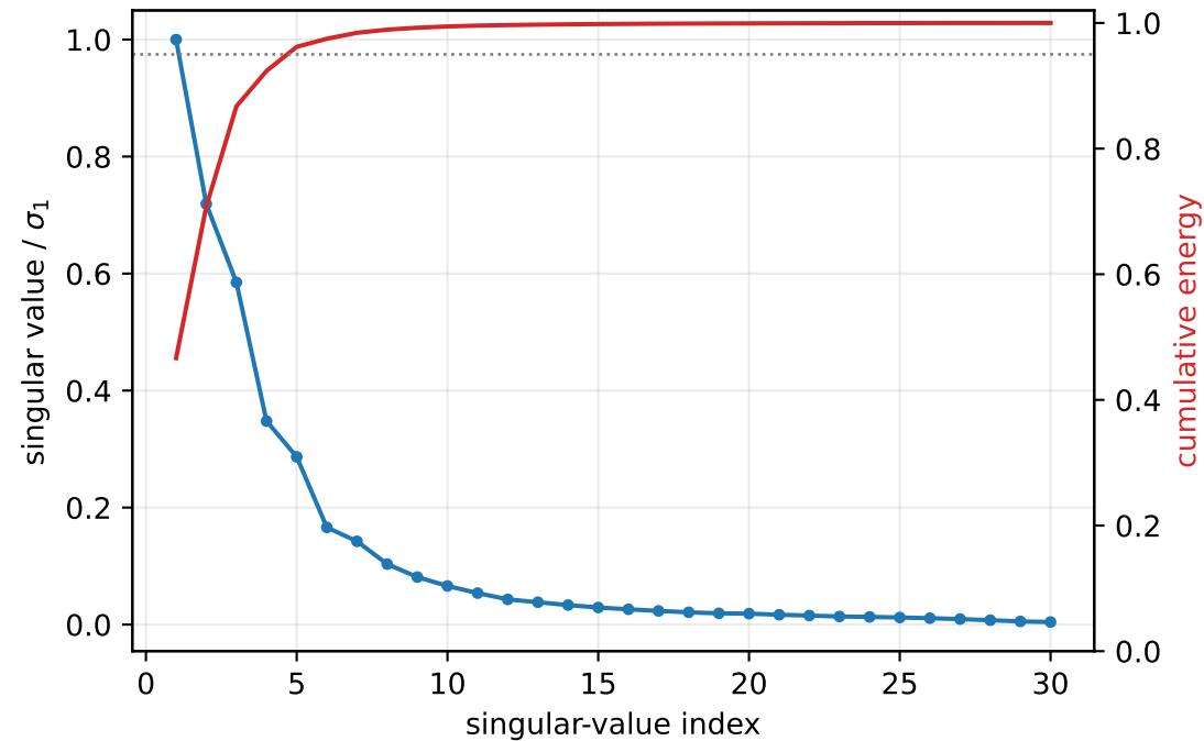
(a) Spectrum of the physical reward ( S=4 ): fast decay
