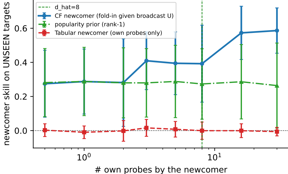
Newcomer cold-start: acts from the broadcast at zero history; tabular newcomer at the floor (Theta(d) vs Theta(n))
