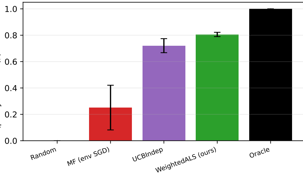
Real simulator: converged skill
