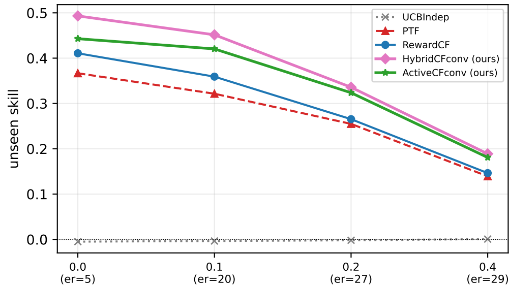
approximate low-rank (entrywise noise)
