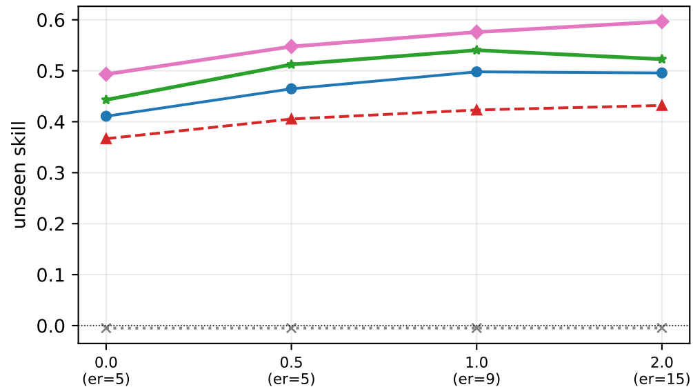
nonlinear reward link
