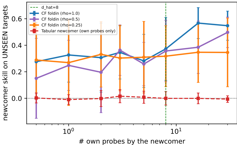
Newcomer cold-start (strict ZK): recovers U from its OWN masked broadcast; tabular at the floor (Theta(d) vs Theta(n)); slope flattens as rho falls
