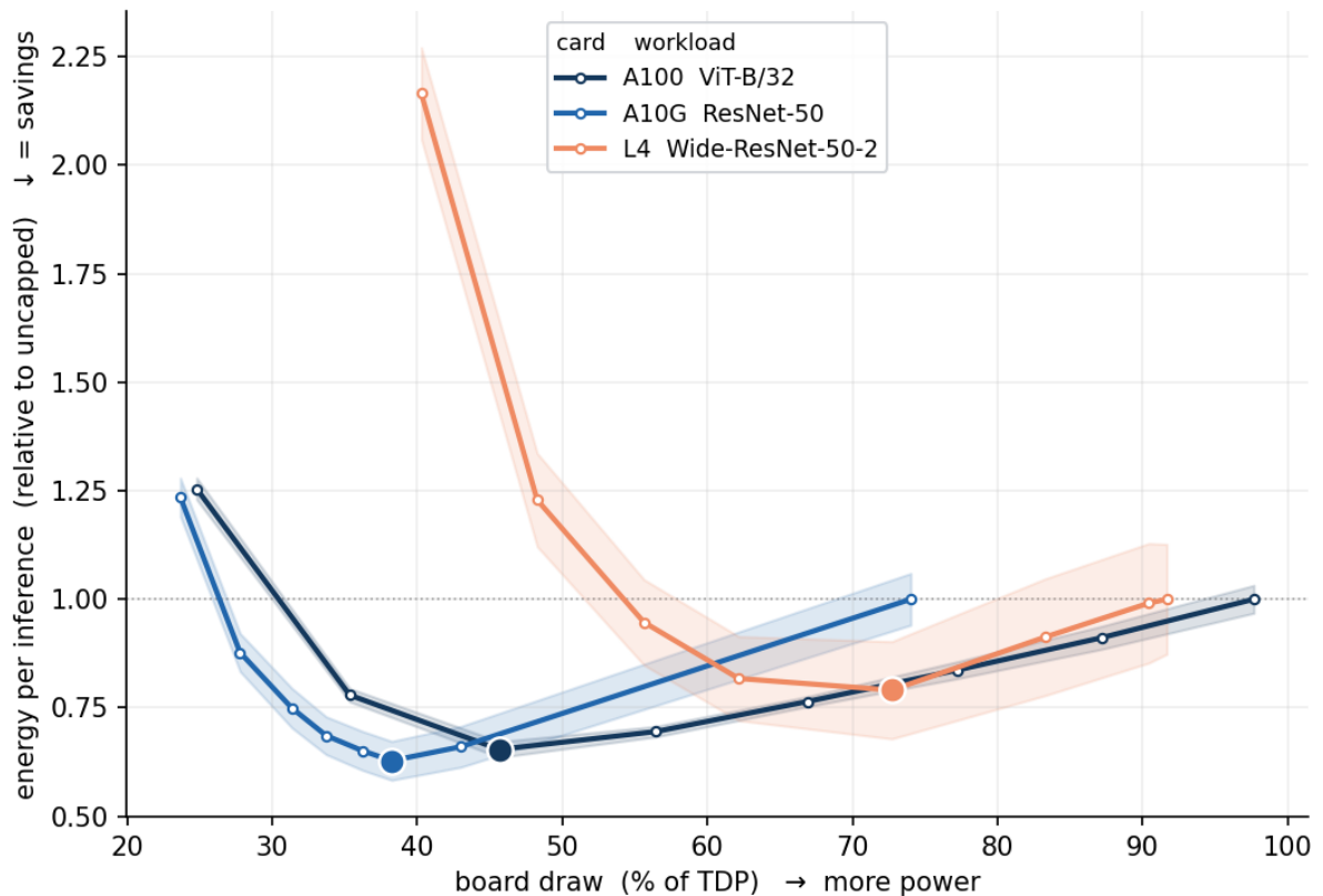
Figure A2. Every card has an energy U-shape. Energy per inference, relative to each card's uncapped value, against board power as a percent of TDP. The dot marks the Joule Point, and the shaded band is one standard deviation over repeats. On the large GPUs the minimum lies
