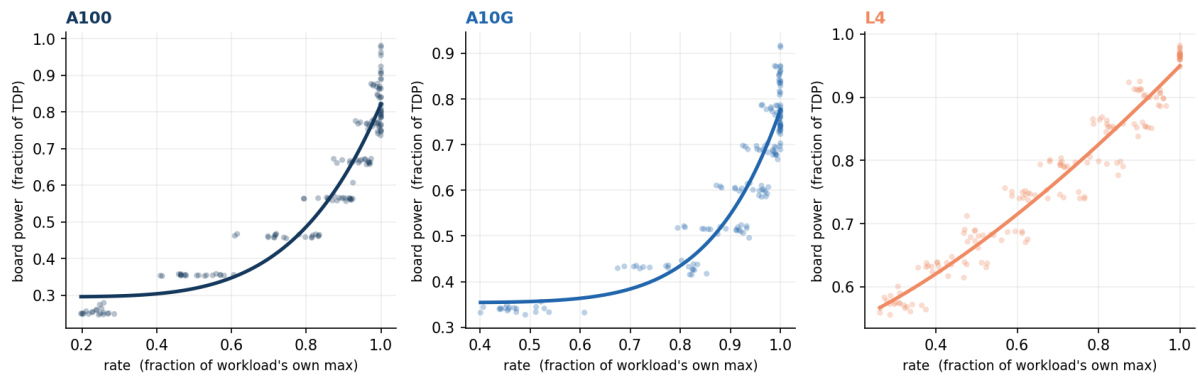
Figure A1. The power curve belongs to the card, not the job. One panel per GPU (A100, A10G, L4). Each dot is one measured operating point for one of the 20 workloads. Rate is scaled to the workload's own maximum, and power to the card's TDP. All 20 workloads on a card follow one fitted law, P(\vartheta) = P_0 + a \cdot \vartheta^b (pooled R^2 0.88 to 0.92 per card, median 0.99 per sweep). This is why one short test per card is enough, which WP2 turns into the transfer model.
