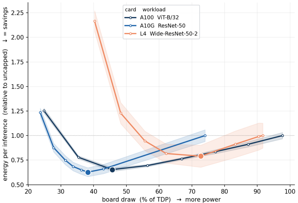
Figure A2. Every card has an energy U-shape. Energy per inference, normalized to each card's own uncapped value, against board draw as a fraction of TDP; the dot marks the JP, the
