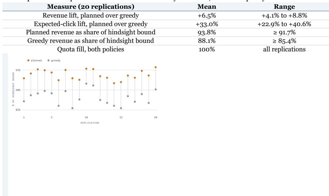
Figure 3. Revenue captured by each policy as a share of the hindsight offline optimum, per replication. Planned allocation dominates greedy serving in all 20 replications; the two distributions do not overlap (planned minimum 91.7%, greedy maximum 91.6%).
