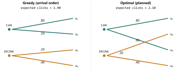
Figure 1. Two campaigns, four subscribers, two impressions per campaign. Greedy serving fills the car campaign with the first arrivals ( u_1, u_2 ) for 0.80 + 0.50 + 0.20 + 0.40 = 1.90 expected clicks. The optimal assignment gives the car campaign u_1 and u_3 and the drink campaign u_2 and u_4 , for 0.80 + 0.60 + 0.30 + 0.40 = 2.10 , an 11% lift from re-pairing the same impressions. The greedy value depends on arrival order; averaged over all orders it is 1.80, so the drawn order is a conservative case.
