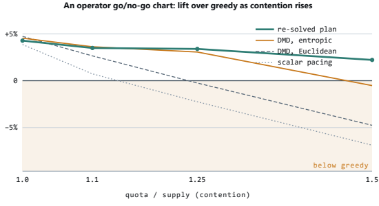
Figure 2. The regime map as a deployment chart. Each curve is one policy’s lift over greedy serving (walk-forward mean, Taobao top-100, pre-committed 8-tier segmentation) as quotas are scaled above deliverable supply. Of the four policies plotted, the re-solved plan is the only one that stays above greedy across the whole contention range; every online price-learning method crosses into the shaded loss region, in order of update aggressiveness (scalar first, then Euclidean, then entropic mirror descent). The static plan and the fixed optimal dual, omitted to keep the chart legible, also stay non-negative under the click objective (Section 6 table). An operator reads the horizontal axis from the pre-deployment contention ratio of Algorithm 1, step 6, and the chart says when planning is worth the effort and which pacing to trust.
