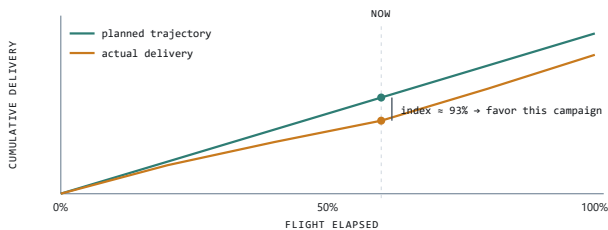
Figure 6. Pacing as trajectory tracking. The plan implies a cumulative delivery path; actual delivery drifts below it, the performance index measures the gap at the current moment, and the decision rule favors the lagging campaign on suitable impressions until the curves reconverge.
