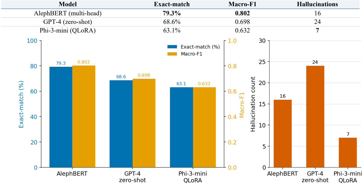
Figure 6. Casualty-record reconstruction: accuracy, F1, and hallucination counts.
