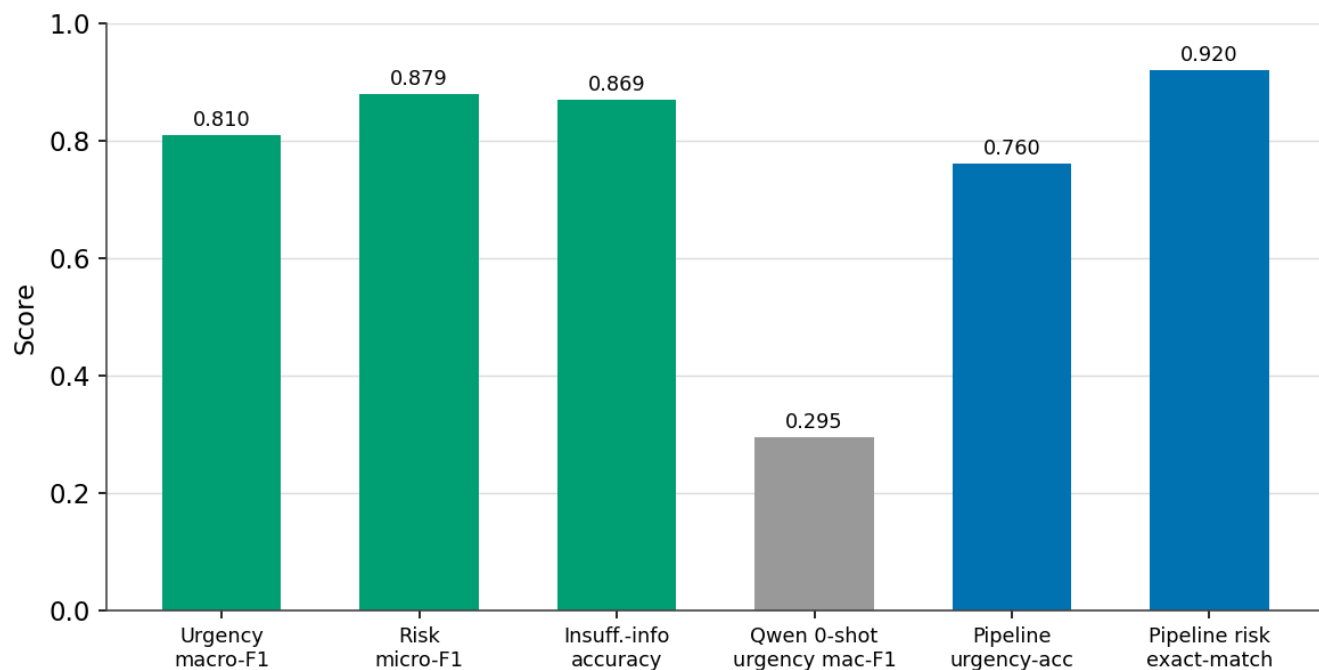
Figure 3. Portal-message triage: fine-tuned heads versus zero- and few-shot prompting.
