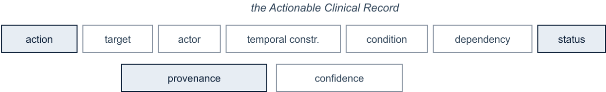
161 162 Figure 2. The ACR schema. Alt text: nine labeled boxes forming the ACR tuple; action , status , 163 and provenance are shaded to mark them as required; target , actor , temporal constraint , condition , de- 164 pendency , and confidence are outlined as optional.
