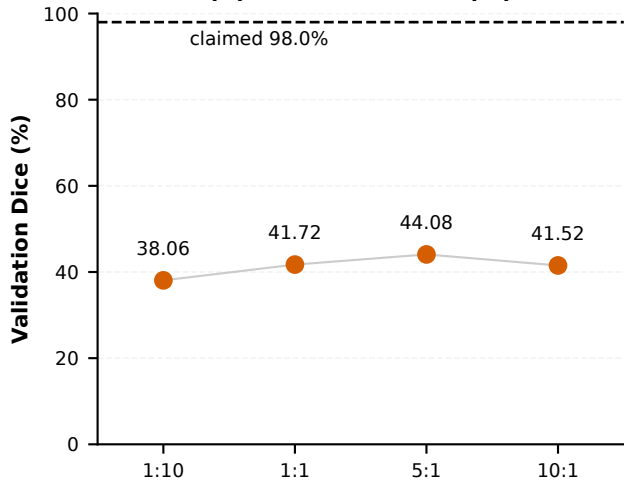
(b) Validation Dice (%)
