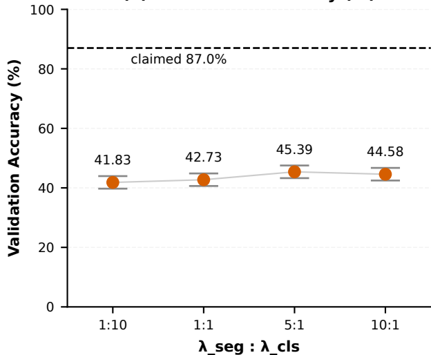
(a) Validation Accuracy (%)
