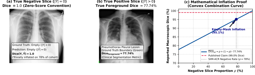
Fig. 1: The empty-mask background-Dice inflation fallacy on sparse medical pathologies (SIIM-ACR pneumothorax). (a) Empty true-negative slice ( |Y| = 0 ) trivially awarded Dice = 1.0 under the zero-score convention despite no lesion present. (b) True-positive slice ( |Y| > 0 , ground truth boundary in green) yielding the true clinical foreground Dice of 77.74%. (c) Analytical convex combination curve (Eq. 5) as a function of negative-slice proportion \rho , showing how 77.74% foreground Dice automatically inflates to 95.10% at \rho = 78\% , reaching > 98\% when negative predictions dominate.
