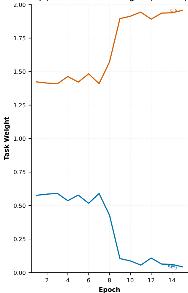
(b) GradNorm task weights (seed 42)
