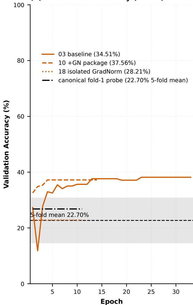
(a) PANDA val. accuracy (fold 1)
