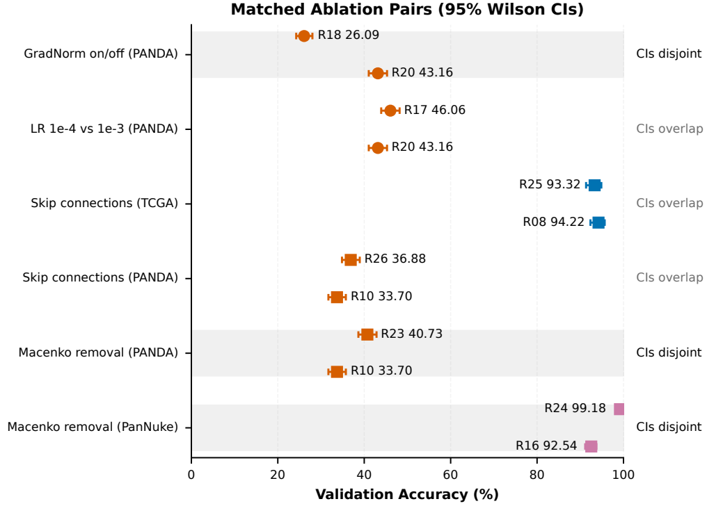
Figure 7: Matched-ablation forest plot of validation accuracy with 95% Wilson CIs for the six strictly matched pairs. Disjoint-CI pairs (shaded): isolated GradNorm (Run 18, 26.09%) vs. static 5:1 (Run 20, 43.16%); no-Macenko PANDA (Run 23, 40.73%) vs. matched (Run 10, 33.70%); no-Macenko PanNuke (Run 24, 99.18%) vs. matched (Run 16, 92.54%). Overlapping-CI pairs: LR 10^{-4} vs. 10^{-3} (Runs 17 vs. 20: 46.06% vs. 43.16%); skip ablation TCGA (Runs 25 vs. 08: 93.32% vs. 94.22%); skip ablation PANDA (Runs 26 vs. 10: 36.88% vs. 33.70%). The right-margin verdict column encodes the CI-overlap test, so the null-result status of the skip ablations and the resolvable Macenko/GradNorm effects are read directly from the plot.
