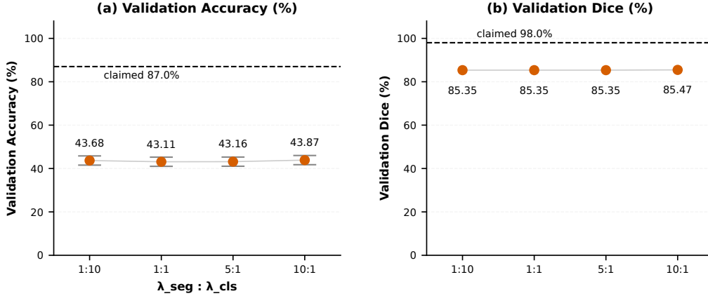
Figure 8: Static loss-weight ratio sweep on PANDA \times VGG16 (raw input, \eta = 10^{-3} , no GradNorm). (a) Validation accuracy with 95% Wilson-CI whiskers: \lambda_{seg} : \lambda_{cls} = 1:10 (43.68%), 1:1 (43.11%), 5:1 (43.16%), 10:1 (43.87%); the black dashed line marks the claimed 87.0% accuracy. (b) Validation Dice for the same four arms (85.35%, 85.35%, 85.35%, 85.47%) against the claimed 98.0%. The ratios yield comparable accuracy (43.11% – 43.87%), yet no ratio approaches the claimed target — the gap is not a loss-weighting artifact.
