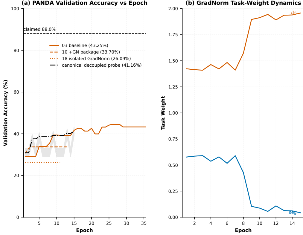
Figure 6: Anatomy of the PANDA accuracy drop. (a) Validation accuracy vs. epoch for three PANDA runs — Run 03 (static 5:1 baseline, 43.25%), Run 10 (v2 GradNorm package, 33.70%), Run 18 (isolated GradNorm at \eta = 10^{-3} , 26.09%) — plus the canonical decoupled GRADNORM probe (dash-dot, shaded 95% CI band), which remains stable but plateaus at 41.16% over 15 epochs, 46.84 percentage points below the claimed 88.0% (black dashed reference). (b) GRADNORM task-weight dynamics from the canonical log: the segmentation and classification weights over 15 epochs, showing the dynamic rebalancing that the joint variant turns into destructive updates on the shared encoder.
