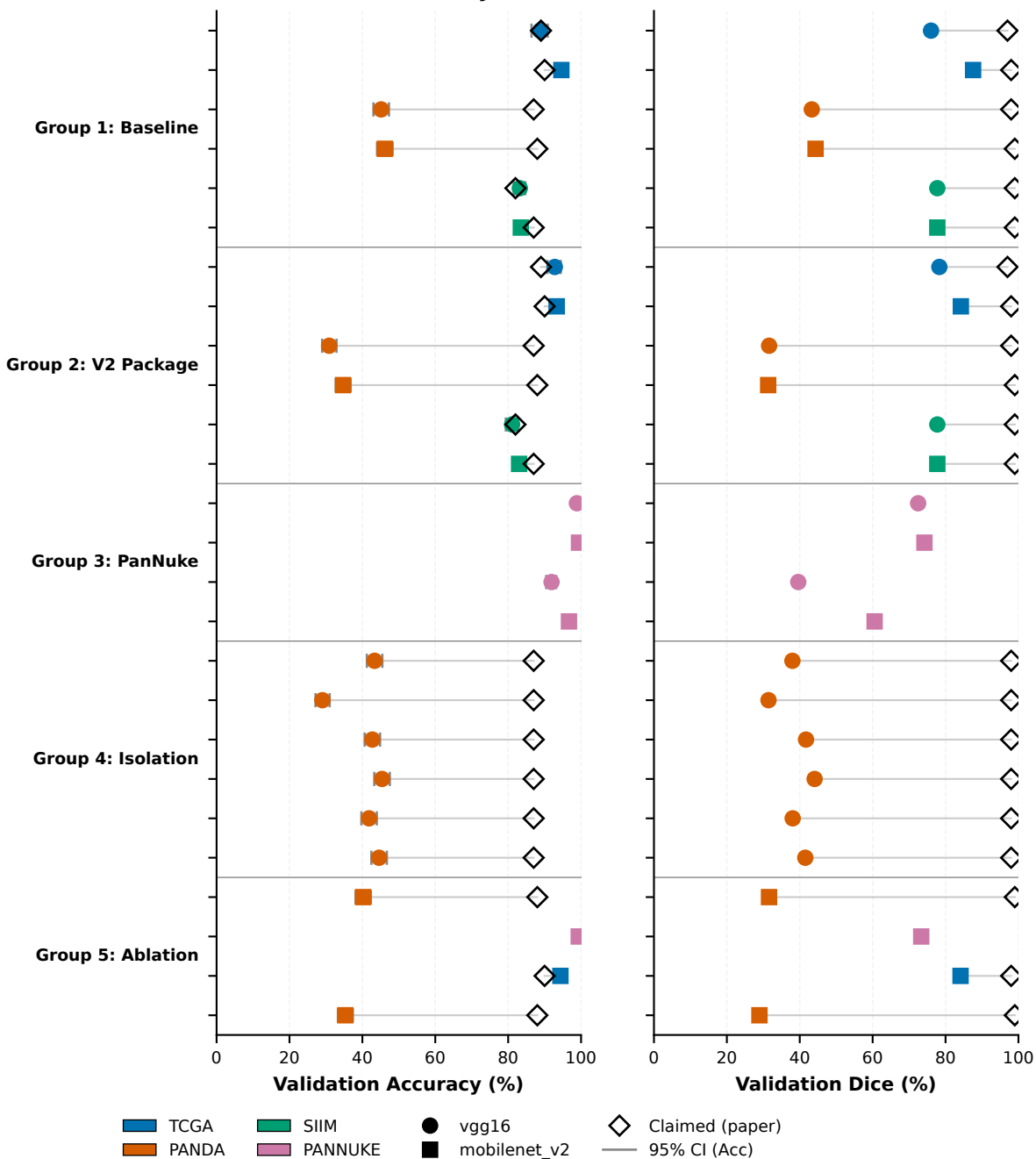
Validation Accuracy (%)
