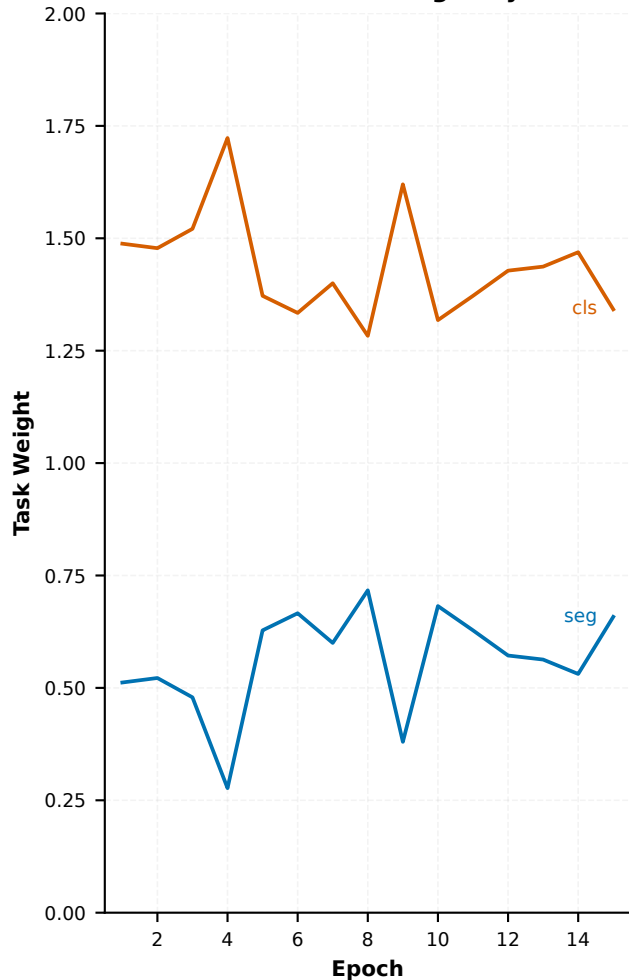
(b) GradNorm Task-Weight Dynamics
