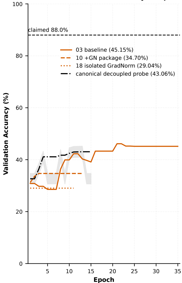
(a) PANDA Validation Accuracy vs Epoch
