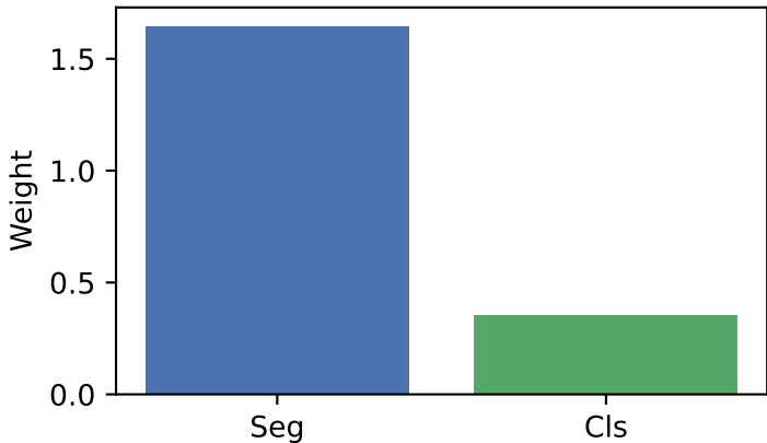
GradNorm weights (final)
