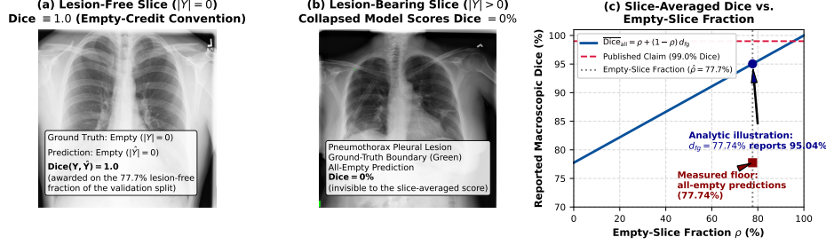
Figure 1: The empty-mask Dice artifact on SIIM-ACR pneumothorax. (a) Lesion-free slice ( |Y| = 0 ): under empty-credit assignment an all-empty prediction is awarded Dice = 1.0; lesion-free slices constitute \hat{\rho} = 77.7\% of our validation split. (b) Lesion-bearing slice ( |Y| > 0 , ground-truth boundary in green): our collapsed models predict empty masks here and score Dice = 0, invisible to the slice-averaged mean. (c) Convex-combination curve (Eq. 6): a foreground Dice of 77.74% would report 95.04% at \hat{\rho} = 0.777 (analytic illustration), whereas all four of our SIIM runs measure the all-empty floor of 77.74% itself.
