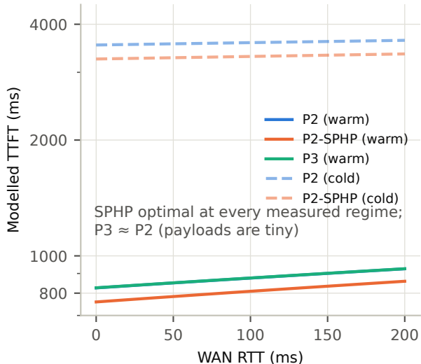
(a) TTFT vs. RTT (BW = 100 Mbps)
