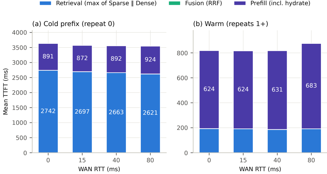
Fig. 7. Mean TTFT composition per regime and cache state (P2 baseline): retrieval barrier (max of the parallel sparse and dense legs), RRF fusion (visually negligible at \approx 0.02 ms), and the prefill residual (hydration + engine prefill + queueing).
