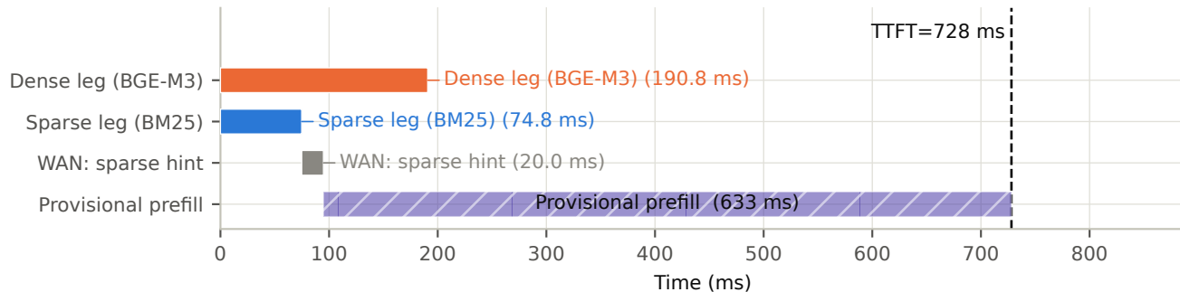
(b) P2-SPHP — provisional prefill overlaps the dense leg (kept on hit)
