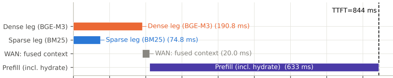
(a) Baseline P2 — serialized (RTT=40 ms, BW=100 Mbps, warm fit)
