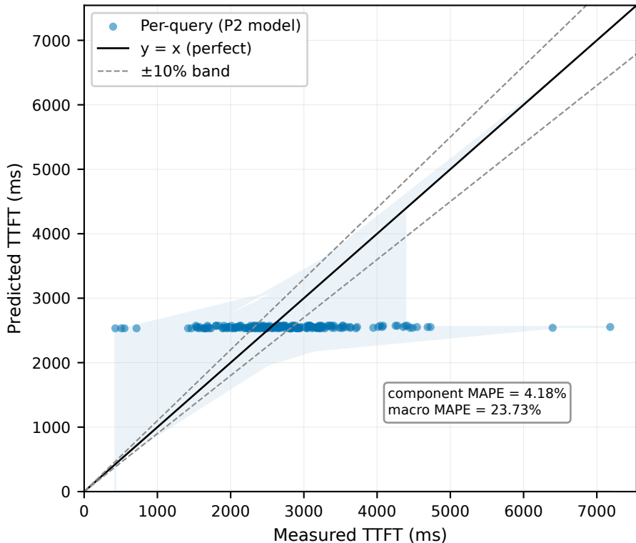
Cost-Model Parity: Predicted vs. Measured TTFT
