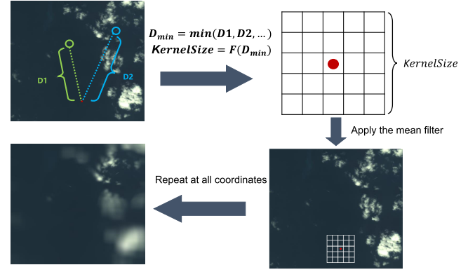
Fig. 3. Specific operation of selective degradation: calculate the mean filter kernel size at each point. D1 and D2 represent the distances from the current pixel position to each ship target, while F(\cdot) is an increasing function to adjust the mean kernel size, where the output, i.e., the mean kernel size, will increase as D_{\min} increases.
