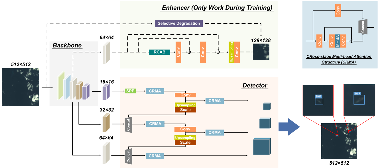
Fig. 2. Overall structure of DRENet. (a) Backbone: a lightweight backbone to enable robust feature extraction efficiently. (b) Enhancer: the proposed DRE to guide the backbone to extract many discriminative features by regressing degraded images. The degraded images come from the proposed “selective degradation” operation. (c) Detector: the detector to display the final detection results. We introduce into the detector a CRMA module, which can gain a large receptive field to locate ships accurately while saving much computation. (For details of RCAB and SPP, please refer to [26] and [27]. The implementations of upsampling layers are aligned with [26] and [27] with nearest-neighbor interpolation in the detector while subpixel convolution in the enhancer.)
