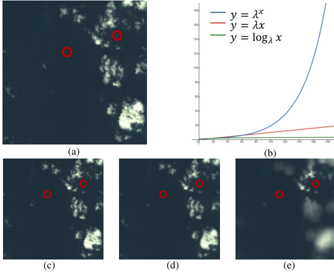
Fig. 8. Degradation effect when takes a logarithmic function, a linear function, and an exponential function to calculate the mean filter kernel size at each position. The red circles in the images are the ships. \lambda is a constant of functions, which is set to ensure that the ship areas are kept clear. (a) Origin images. (b) Different functions F(\cdot) . (c) y = \log_\lambda x . (d) y = \lambda x . (e) y = \lambda^x .
