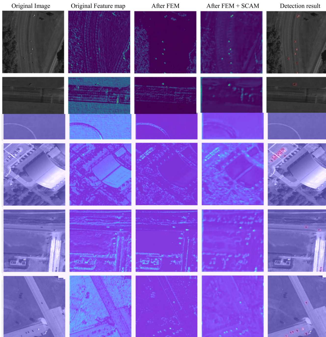
Fig. 11. Influence of FEM and SCAM on feature extraction. The brighter color represents that the model pays more attention to that area.
