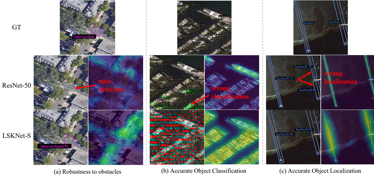
Figure 6. Eigen-CAM visualization of Oriented RCNN detection framework with ResNet-50 and LSKNet-S. Our proposed LSKNet can model a much long range of context information, leading to better performance in various hard cases.
