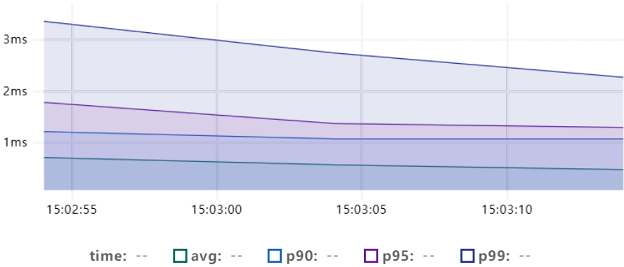
Request Connecting
