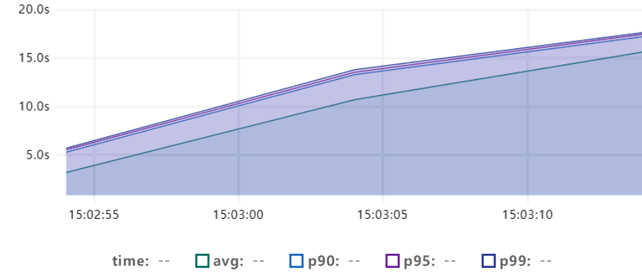
Request Waiting
