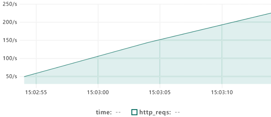
Request Rate
