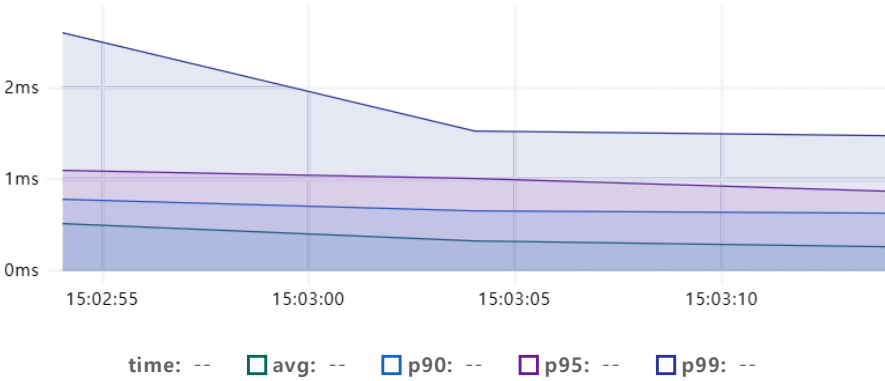
Request Receiving
