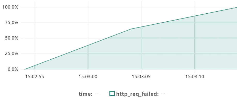
k6 report
