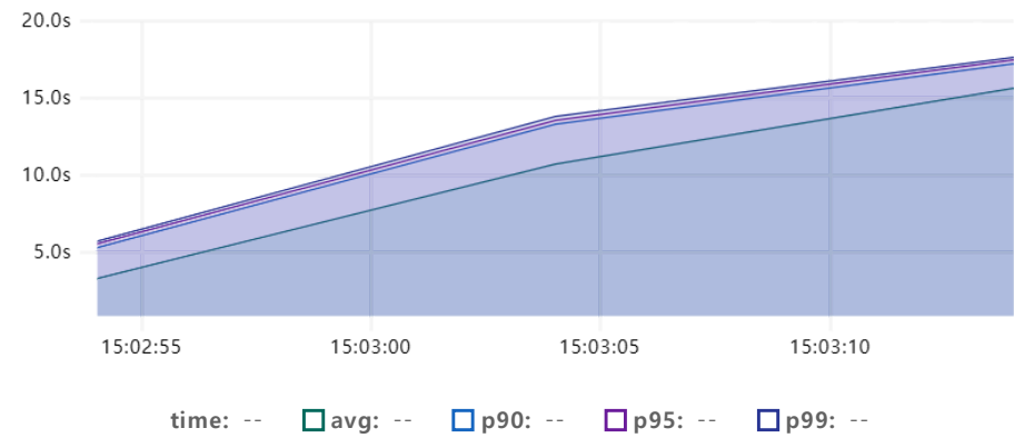
Iteration Duration
