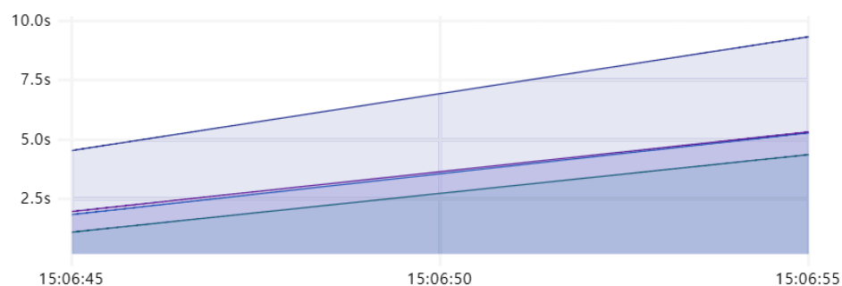
HTTP Request Duration
