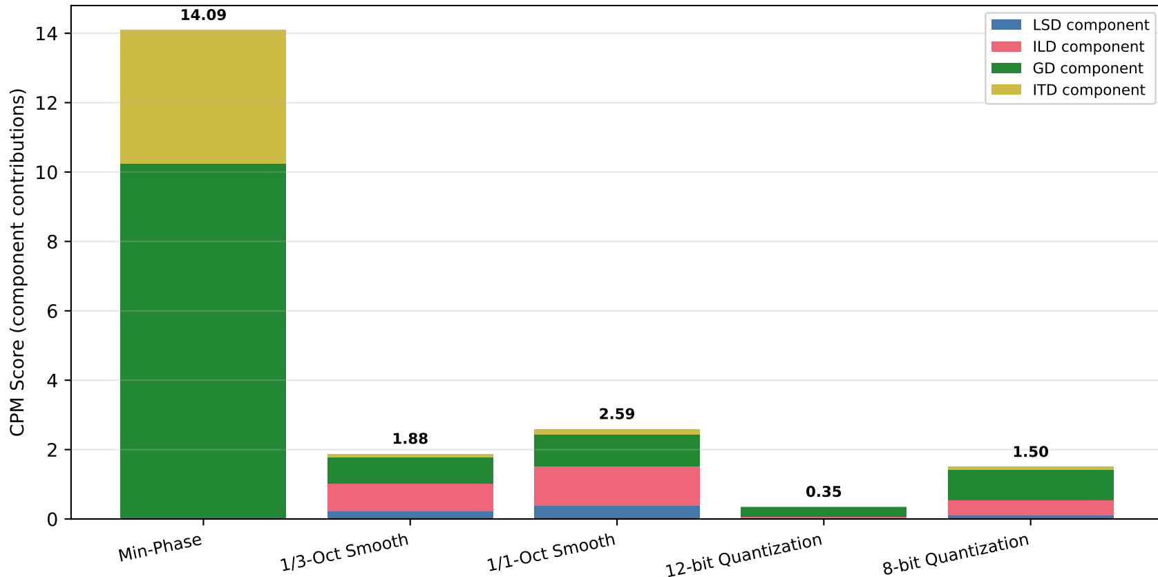
Figure 4.7 — CPM Component Breakdown by Degradation Condition Group delay dominates the Min-Phase condition score
