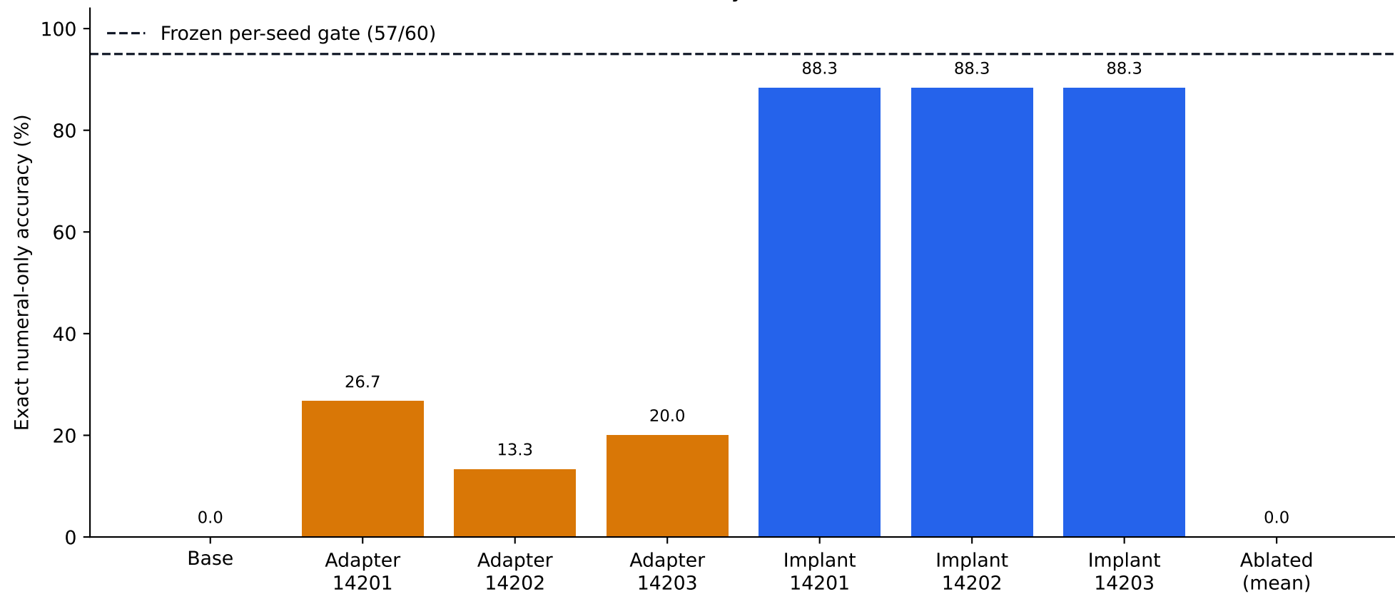
Phase 8 frozen TinyLlama confirmation
