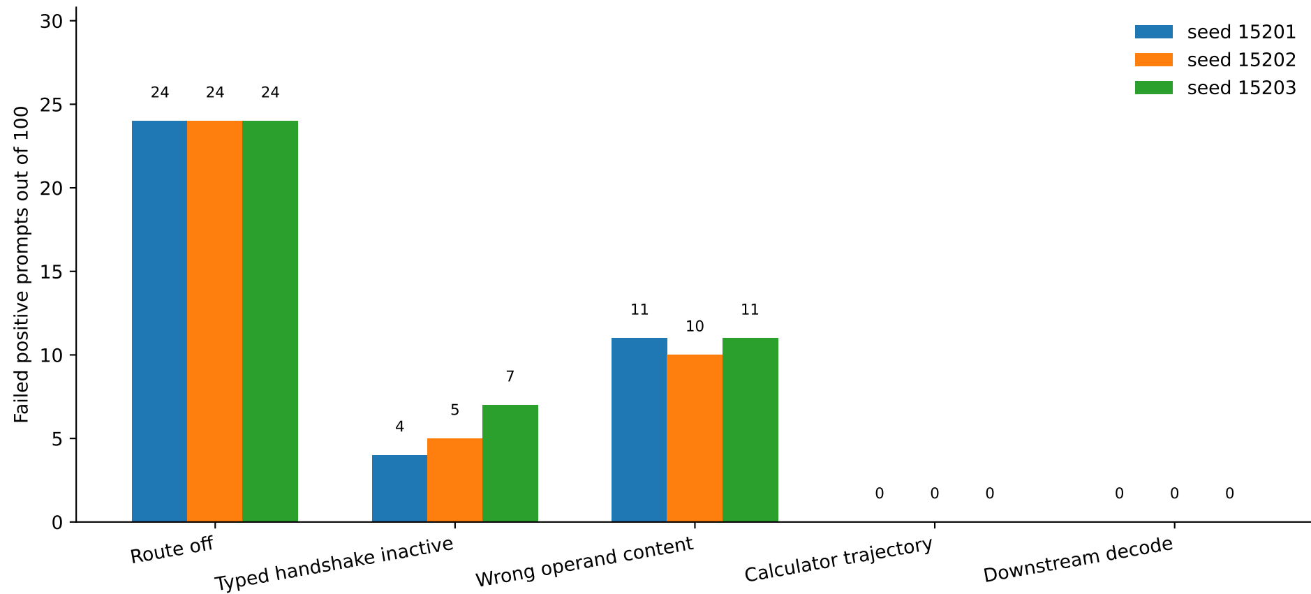
Where Phase 9 hard-condition failures occur
