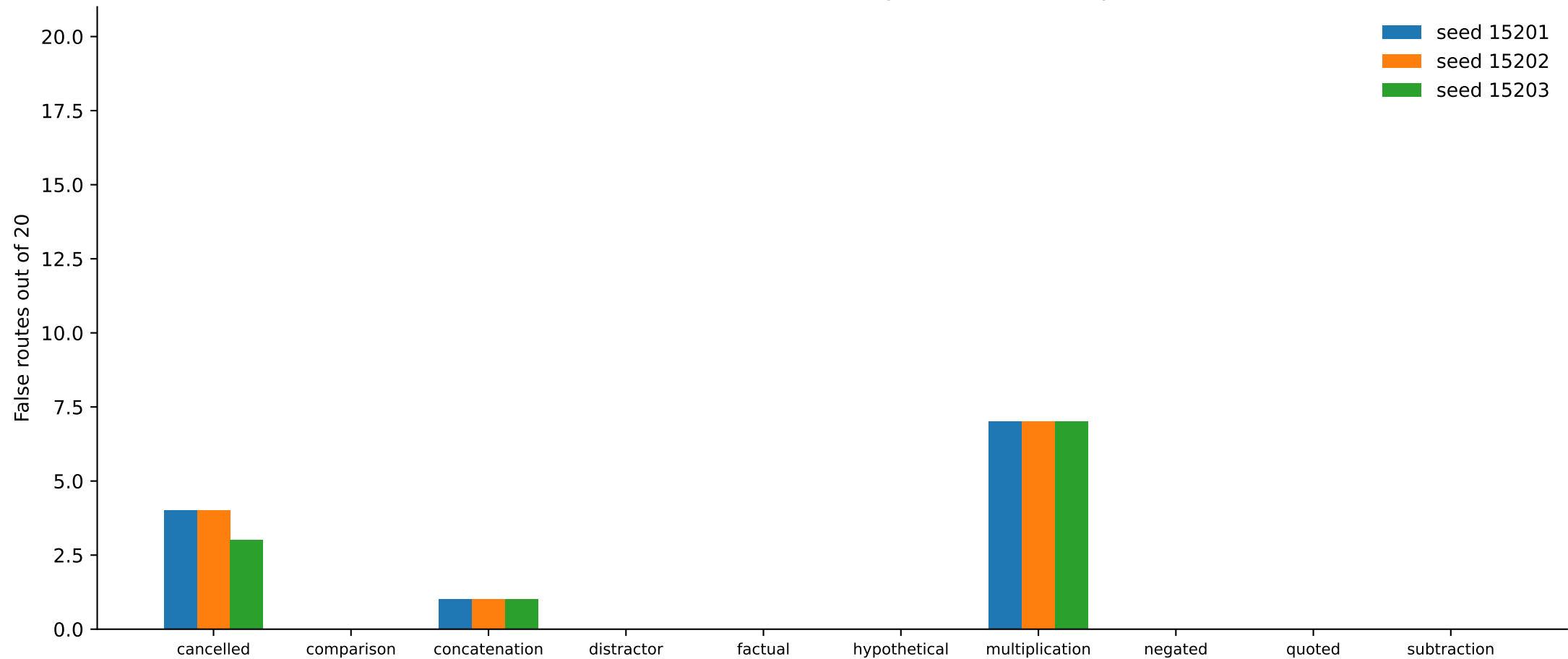
Hard-condition false routes by adversarial family
