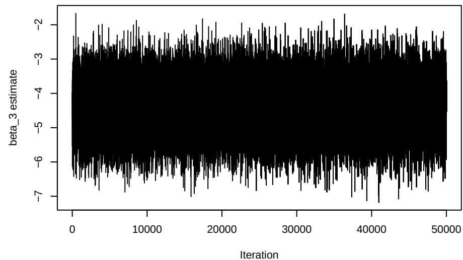
Trace Plot of Posterior Samples for \beta_3
