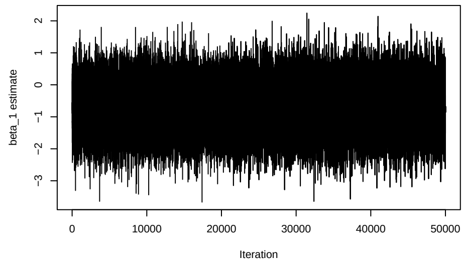
Trace Plot of Posterior Samples for \beta_1
