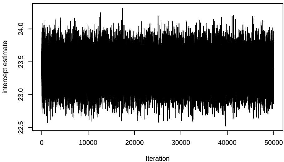
Trace Plot of Posterior Samples for \beta_0
