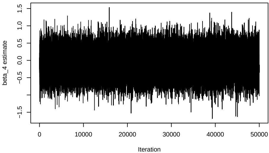
Trace Plot of Posterior Samples for \beta_4
