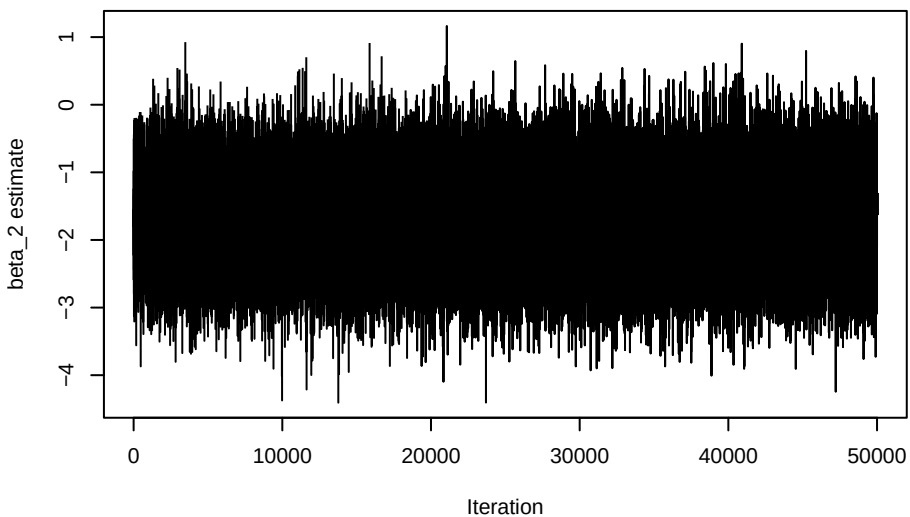
Trace Plot of Posterior Samples for \beta_2
