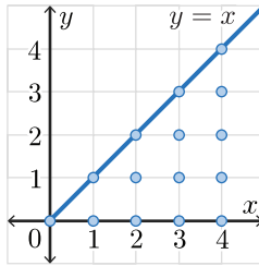
Figure 4.6.2: Set of (x, y) points where the joint pmf of (X, Y) is defined for Example 4.6.3
