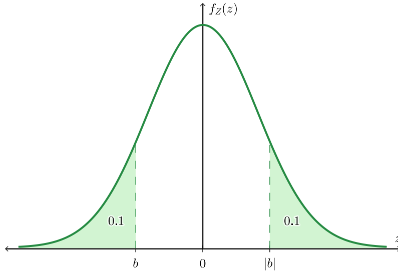
Figure 5.4.7: Useful picture in helping to find b satisfying P(Z > b) = 0.9 in Example 5.4.3
