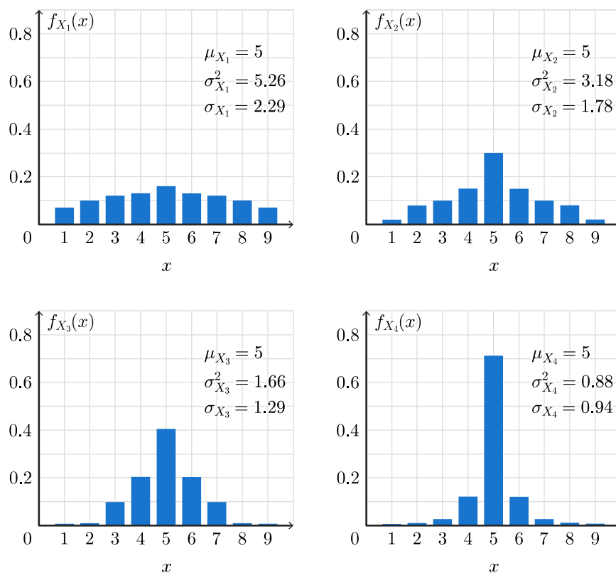
Figure 3.3.3: Comparison of variability over four discrete probability distributions
