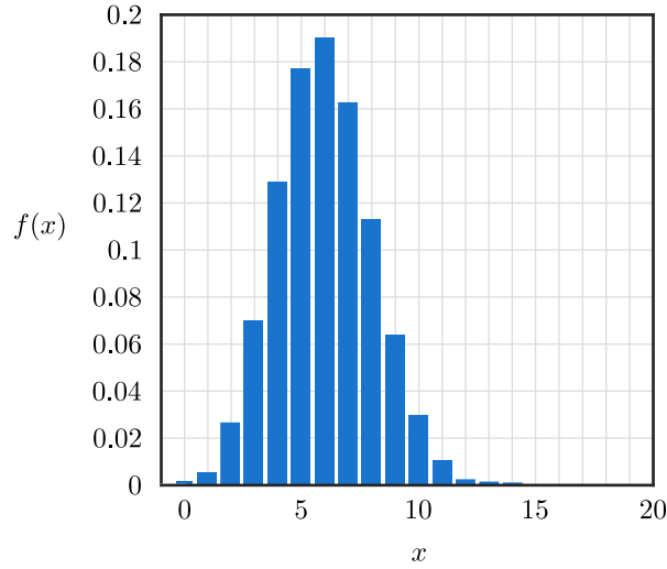
Figure 3.5.1: Probability histogram for a \text{Bin}(20, 0.3) random variable
