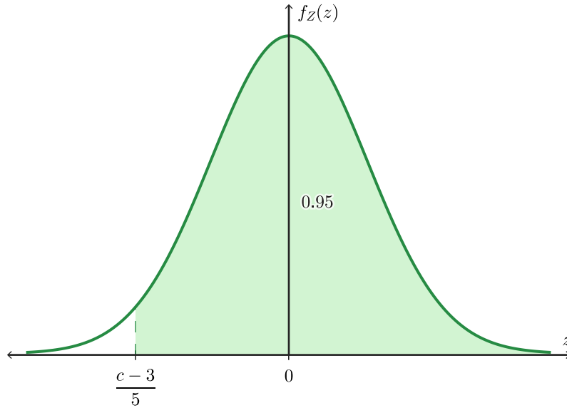
Figure 5.4.9: Useful picture in helping to find c satisfying P\left(Z > \frac{c-3}{5}\right) = 0.95 in Example 5.4.4
