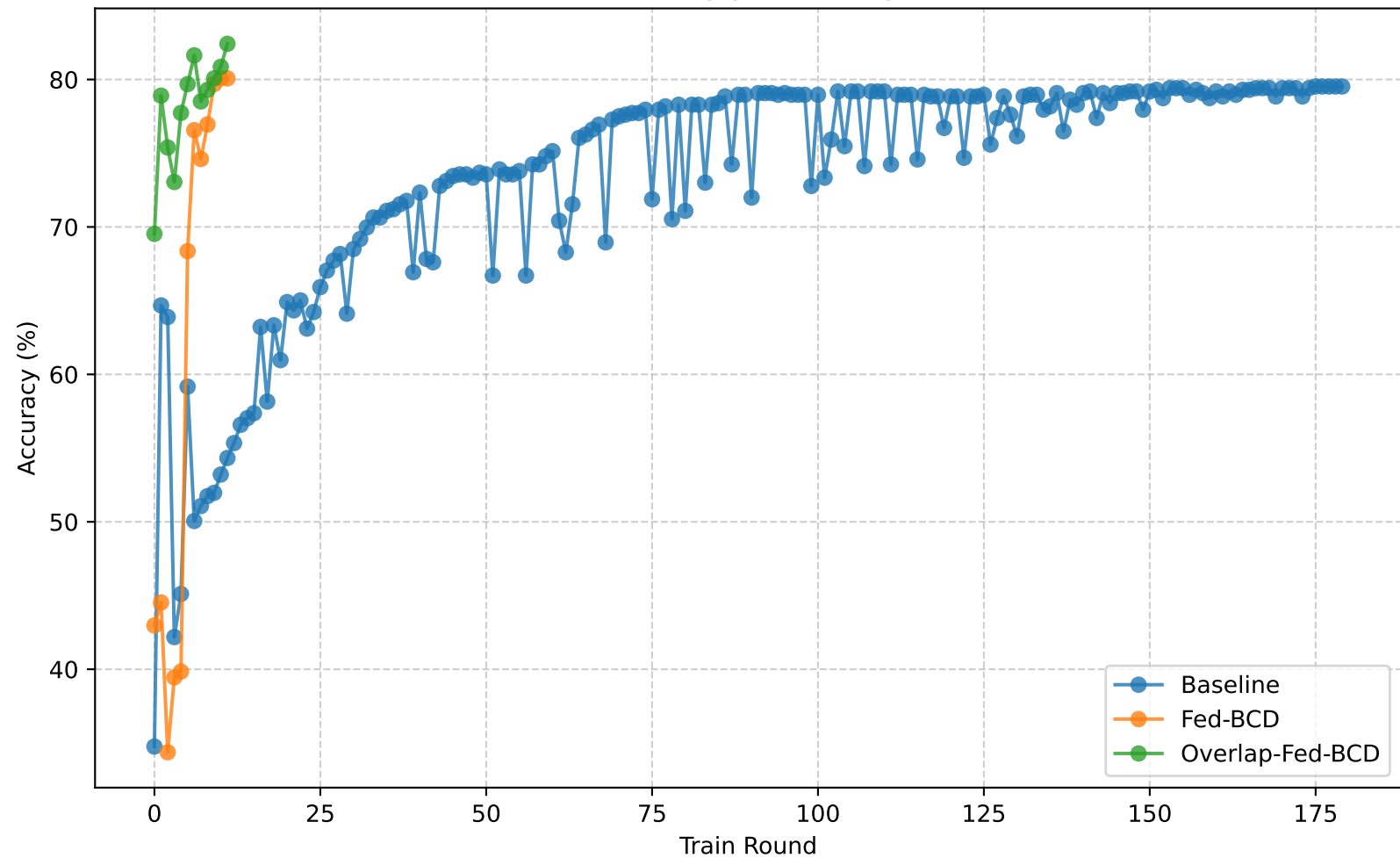
Model Accuracy per Training Round
