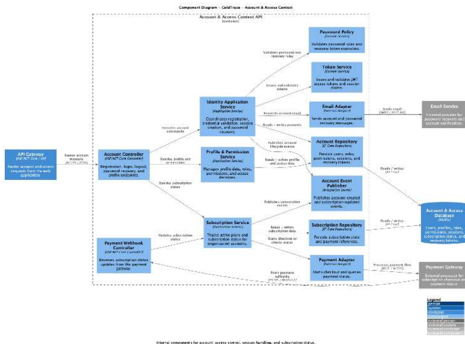
Figura 4.6.4.1. Component Diagram del Account & Access Context.
